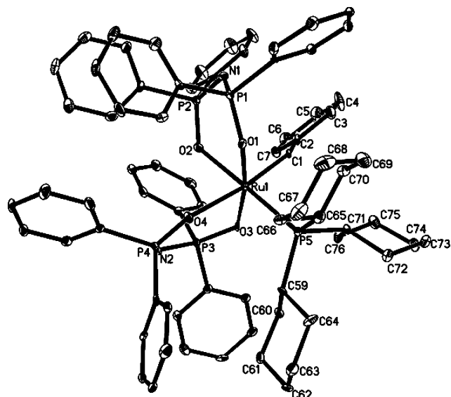
Figure 7. Molecular structure of cis -Ru(tpip) 2 (CHPh)(PCy 3 ) ( 9 ). The ellipsoids are drawn at the 30% probability level.
